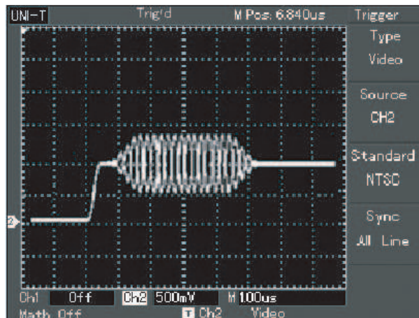
Figure 2-14 Video trigger: line synchronization
