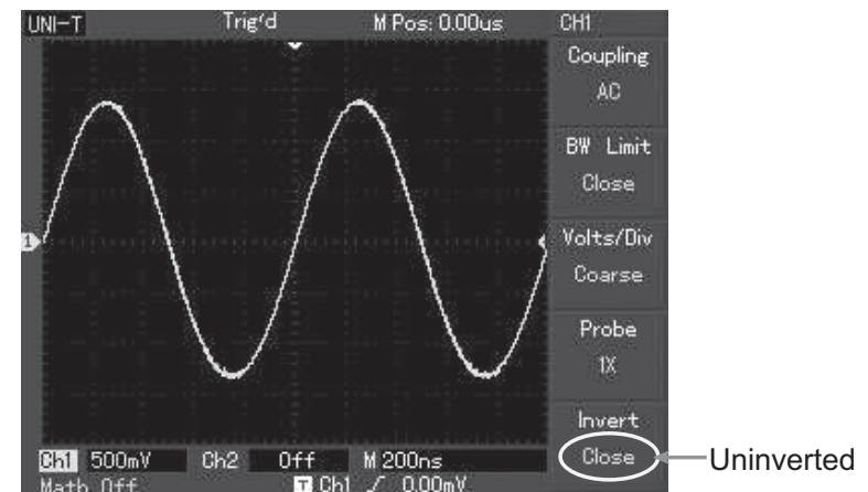
Figure 2-8 Inversion setup for vertical channel inversion (uninverted)
